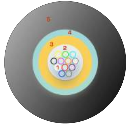
1. Fibers 2. Filling 3. Aramid Yarn 4. Loose Tube 5. Outer
